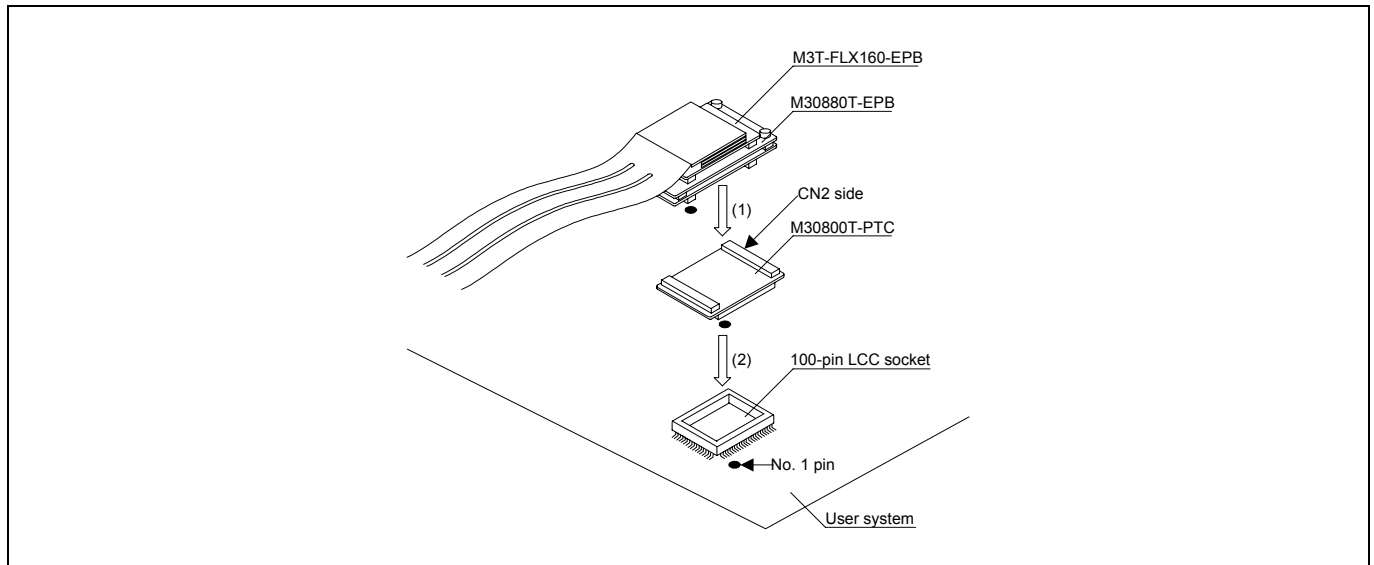
Figure 2.8 Connecting to a 100-pin LCC socket
